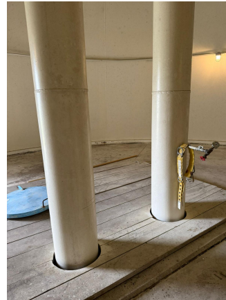
Lower Portion of Fill Line within Conical Base
